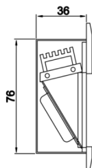
Technical Drawing
