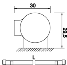
Technical Drawing
