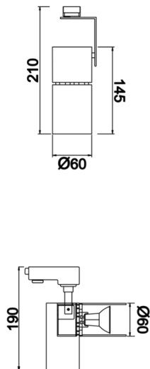
Technical Drawing
