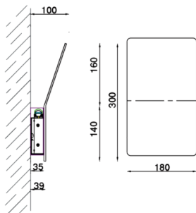
Technical Drawing
