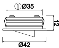
Technical Drawing
