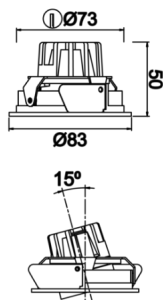
Technical Drawing
