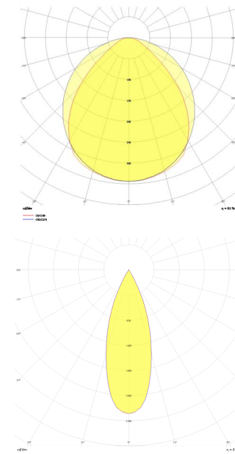
Photometric Curve
