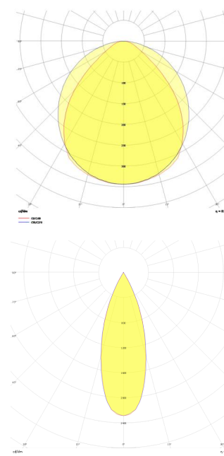
Photometric Curve
