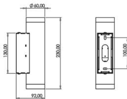
Technical Drawing
