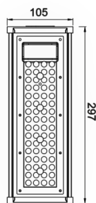
Technical Drawing
