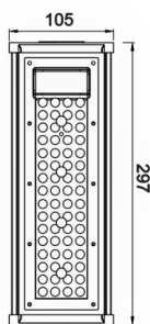
Technical Drawing
