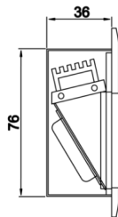
Technical Drawing
