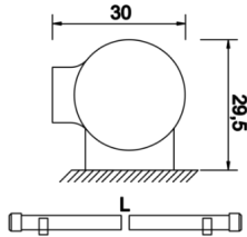
Technical Drawing
