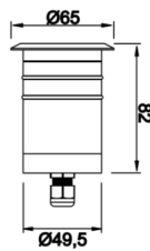
Technical Drawing
