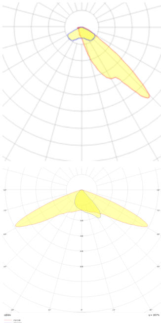
Photometric Curve
