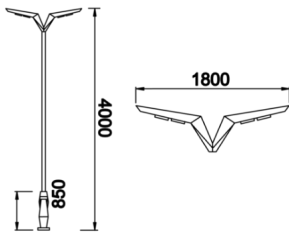
Technical Drawing
