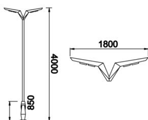
Technical Drawing
