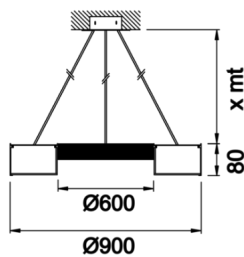
Technical Drawing
