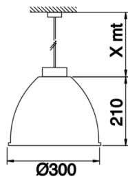
Technical Drawing
