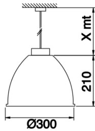
Technical Drawing
