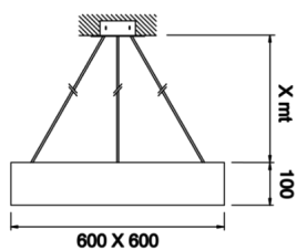
Technical Drawing
