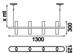
Technical Drawing
