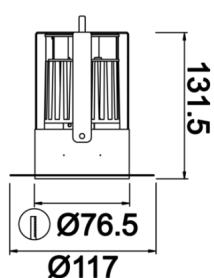
Technical Drawing
