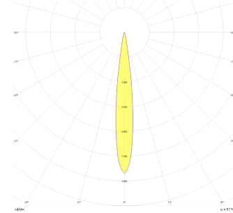
Photometric Curve
