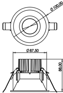
Technical Drawing
