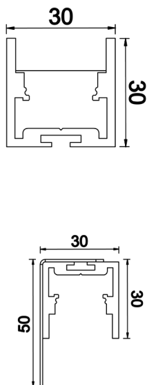
Technical Drawing
